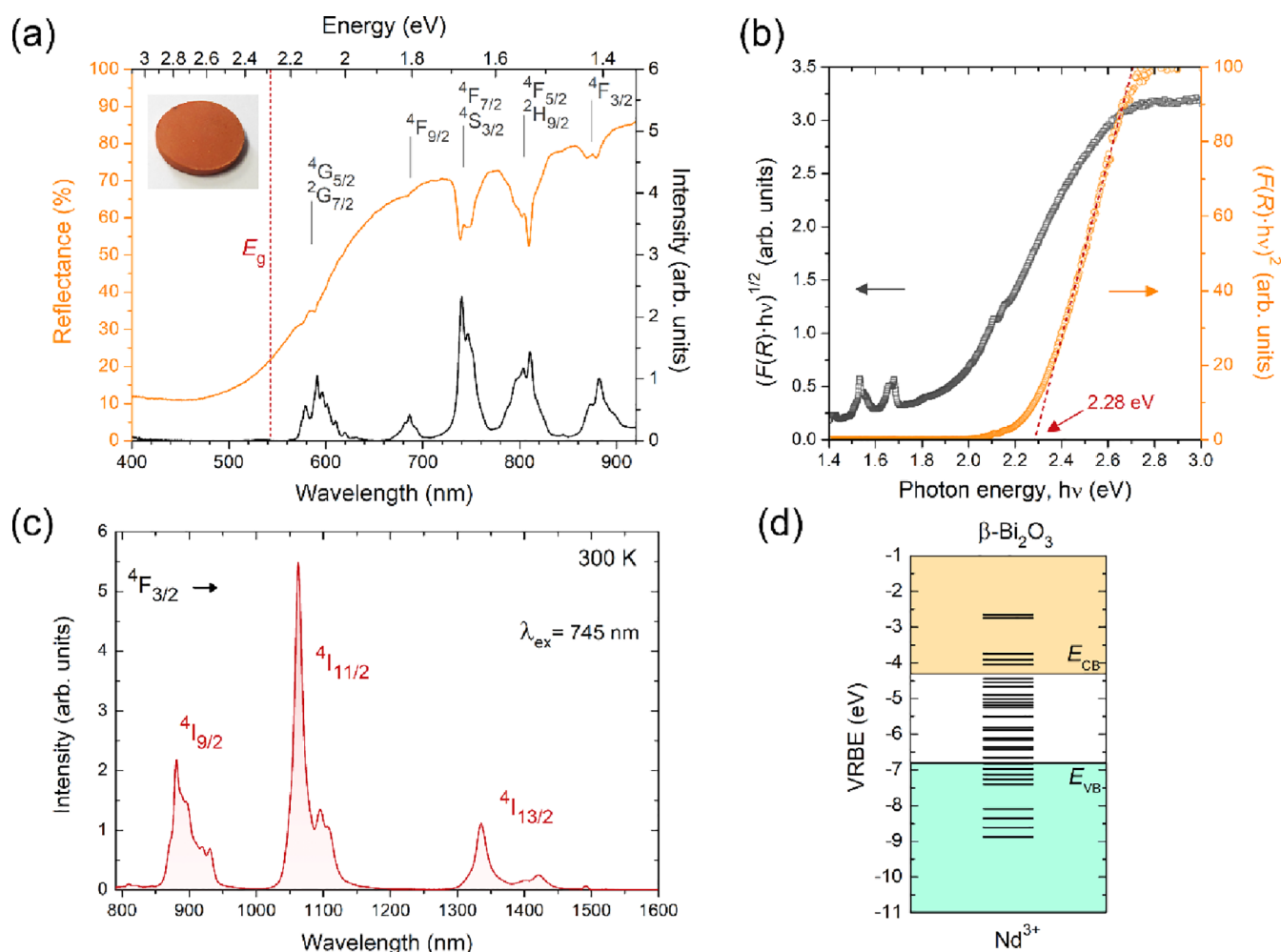
Figure 2. Electronic structure and optical properties of the narrow band gap \beta\text{-Bi}_2\text{O}_3\text{:Y}^{3+},\text{Nd}^{3+} . (a) Reflectance and PLE spectra collecting at 1060 nm along with the picture of the sample. (b) Tauc plot of the Kubelka–Munk function F(R) for the estimation of the band gap energy. (c) Room temperature PL spectrum by exciting at 745 nm. (d) VRBE diagram for \text{Nd}^{3+} in \beta\text{-Bi}_2\text{O}_3\text{:Y}^{3+},\text{Nd}^{3+} .
