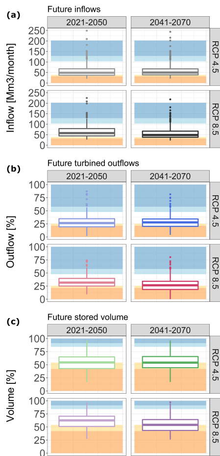
Figure 5. Thirty-year slice boxplots for future projections of (a) simulated water inflow to the S. Giustina reservoir, (b) simulated turbinized water and (c) simulated future water volume stored in the S. Giustina reservoir. Coloured bands outline areas of baseline values lower than the 10th and 20th and greater than the 80th and 90th percentiles using the same colours as in Fig. 4. For an interpretation of the references to colour in this figure legend, the reader is referred to the web version of this article.
