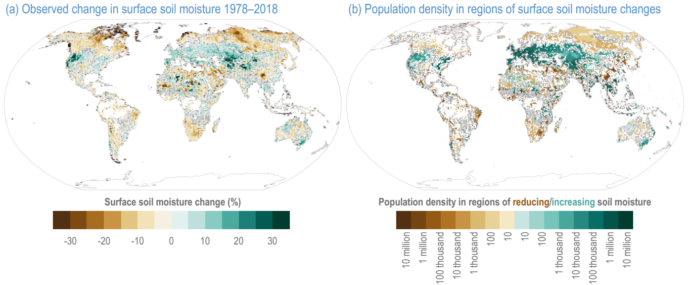
Figure 4.4 | Global patterns of changes in surface soil moisture and people in regions with significant changes.
