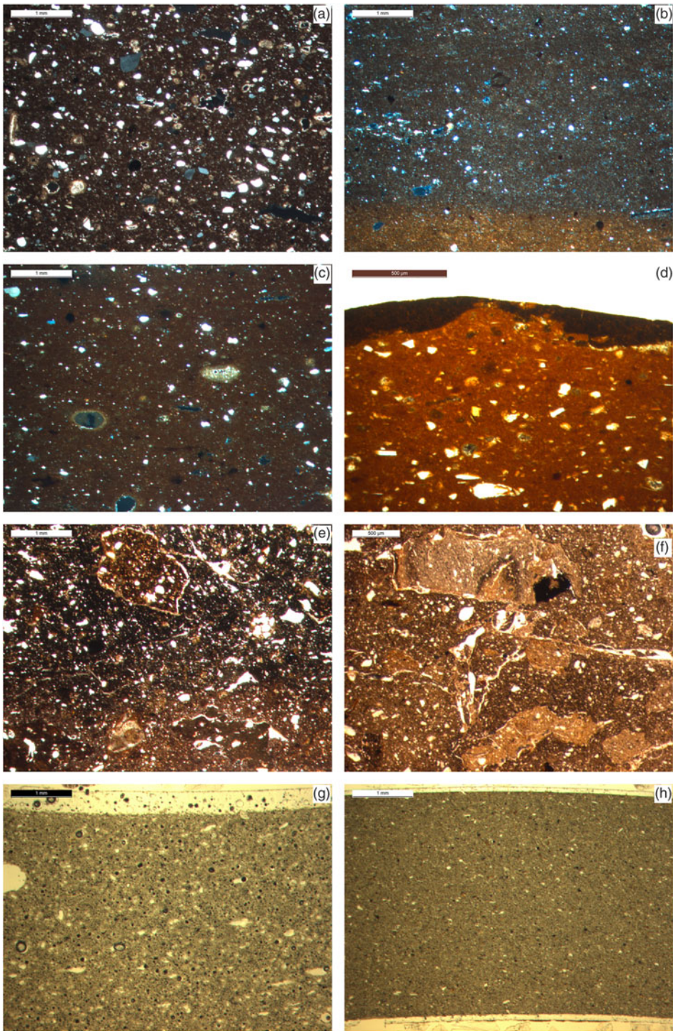
Fig 18. Sonari: photomicrographs of ceramic thin sections of samples. a) SNR4; b) SNR5; c) SNR8; d) SNR13; e) SNR12; f) SNR14; g) blue-on-white SNR102; h) SNR101 white porcelain samples. Photomicrographs a–c were taken in cross polarised light, and d–h in plane polarised light. Photographs: M Spataro.
