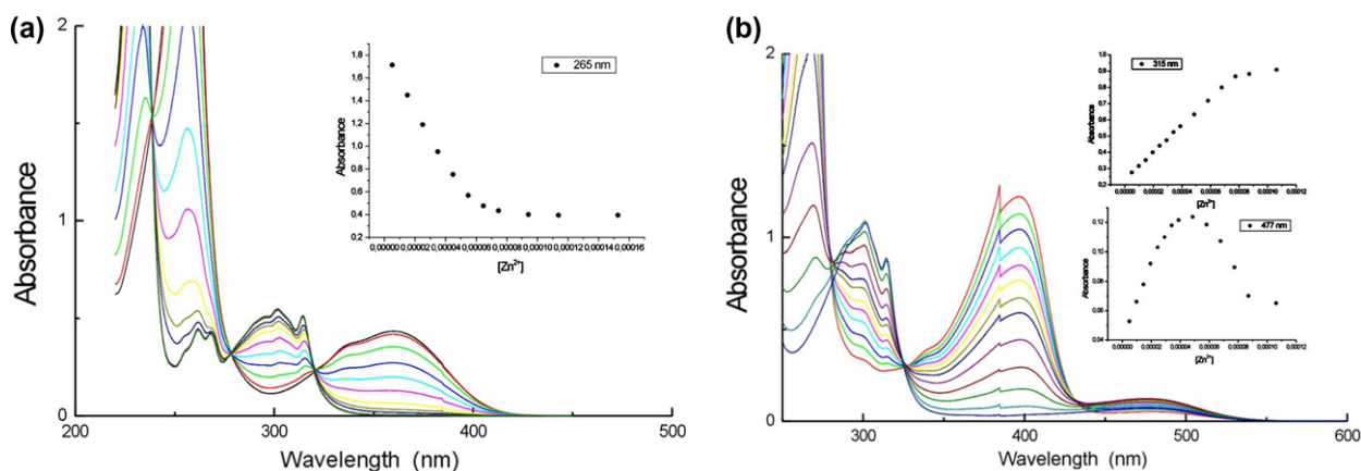
Fig. 4. Absorbance changes upon addition of \text{Zn}(\text{ClO}_4)_2 to an acetonitrile solution of NNN(Qui) (a) and BQAH (b) ([Ligand] = 1 \times 10^{-4} mol dm -3 ).
