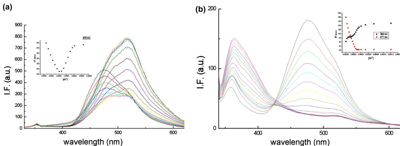
Fig. 6. Fluorescence spectra of acetonitrile solutions of NNN(Qui) ( 4.3 \times 10^{-5} \text{ mol dm}^{-3} ; \lambda_{\text{exc}} = 321 \text{ nm} , slit 5/5) (a) and BQAH ( 3 \times 10^{-5} \text{ mol dm}^{-3} ; \lambda_{\text{exc}} = 321 \text{ nm} , slit 5/5), (b) upon addition of \text{Zn}(\text{ClO}_4)_2 ( 0.005 \text{ mol dm}^{-3} ).
