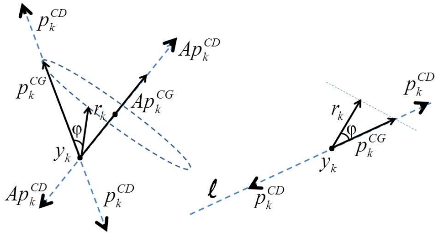
Figure 1: At the k th iteration of the CG and CD, the directions p_k^{CG} and p_k^{CD} are respectively generated, along the line \ell . Applying the CG, the vectors p_k^{CG} and r_k have the same orthogonal projection on Ap_k^{CG} , since (p_k^{CG})^T Ap_k^{CG} = r_k^T Ap_k^{CG} . Applying CD, the latter equality with p_k^{CD} in place of p_k^{CG} is not necessarily satisfied
