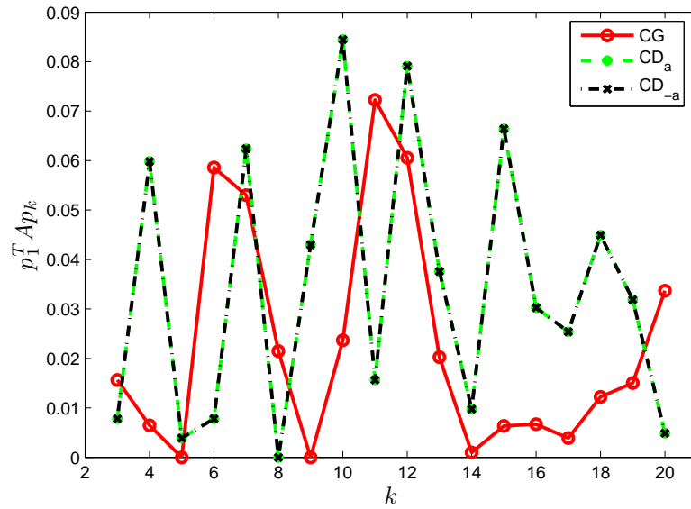
Figure 3: Conjugacy loss for an illconditioned problem described by the coefficient matrix A_{1_0} in [13], using only the CG, CD_a (the CD class setting \gamma_0 = 1 and \gamma_k = a_k , k \geq 1 ) and CD_{-a} (the CD class setting \gamma_0 = 1 and \gamma_k = -a_k , k \geq 1 ). The quantity p_1^T A p_k is reported for k \geq 3 . The choices \gamma_k = a_k and \gamma_k = -a_k are definitely comparable, and are preferable to the CG for k \in \{3, 6, 8, 11, 20\} .
