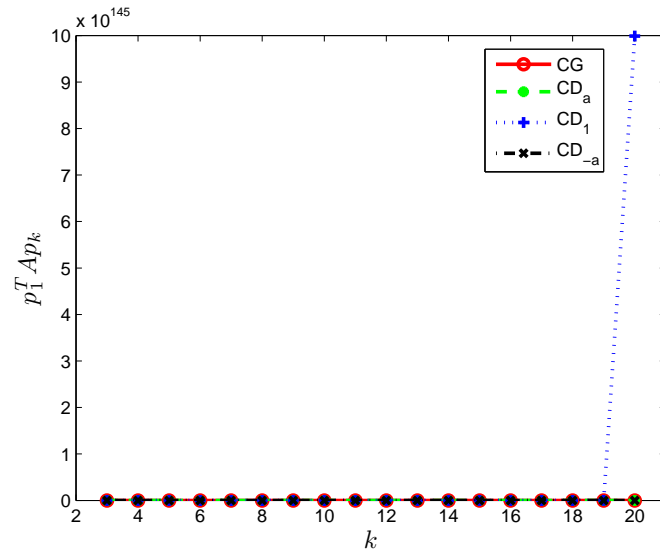
Figure 2: Conjugacy loss for an illconditioned problem described by the coefficient matrix A_{1_0} in [13], using the CG, CD_a (the CD class setting \gamma_0 = 1 and \gamma_k = a_k , k \geq 1 ), CD_1 (the CD class setting \gamma_k = 1 , k \geq 0 ) and CD_{-a} (the CD class setting \gamma_0 = 1 and \gamma_k = -a_k , k \geq 1 ). The quantity p_1^T A p_k is reported for k \geq 3 . As evident, the choice \gamma_k = 1 , k \geq 0 , can yield very harmful results when the coefficient matrix is illconditioned
