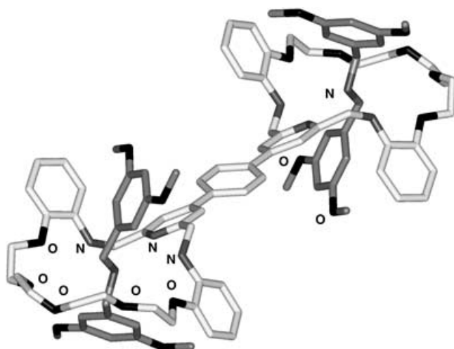
Figure 8. Solid-state structure of the bis[2]rotaxane [\mathbf{17}\text{-H}_2][\text{PF}_6]_2 .
