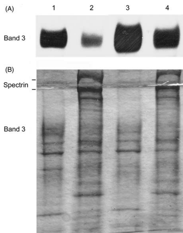
Figure 4 Phosphorylation pattern of Triton-soluble and cytoskeletal band 3 Tyr-phosphorylation by p72 Syk and p36 Syk . Isolated membranes (15 \mu g) were incubated with p72 Syk (20 ng) (lanes 1 and 2) or p36 Syk (10 ng) (lanes 3 and 4) in the reaction mixture (see 'Materials and Methods') for 10 min at 30°C. After washing to remove unincorporated radionucleotide, both samples were then treated with Triton X-100 (1% final concentration) for 5 min at 0°C and centrifuged at 80,000 g for 40 min. Pelleted insoluble residues were resuspended in Tris buffer to same starting volume. Fractions of both Triton extract (lanes 1 and 3) and cytoskeleton (lanes 2 and 4) were analyzed by SDS-PAGE and either western blotting analysis and immunorevelation with anti P-Tyr antibody (A) or Coomassie Blue staining (B).
