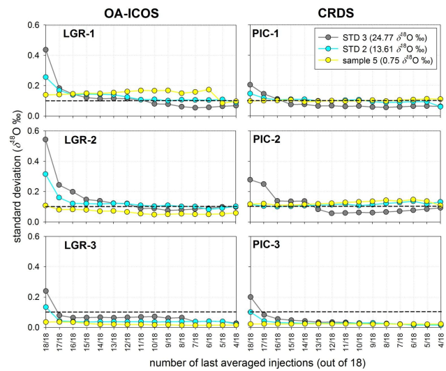
Fig. 4b. Standard deviation for \delta^{18}\text{O} for two laboratory measurement standards and one sample as a function of number of averaged injections. 18/18 indicates that all 18 injections of the same vial (either standard or sample) were averaged, whereas 17/18, 16/18, 15/18... indicates that only the last 17, 16, 15... injections were averaged (and the remaining discarded). The dotted horizontal line indicates an acceptable reference precision for \delta^{18}\text{O} (0.1 ‰). The legend depicts the difference between the isotopic composition of the standard/sample displayed and the isotopic composition of the previous vial analysed in the tray.
