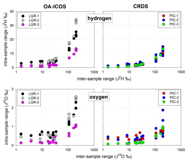
Fig. 3. Relation between the isotopic range (maximum–minimum of 18 injections) within each vial (either sample or measurement standard) and the absolute isotopic difference between adjacent vials in the tray. Upper row: hydrogen. Lower row: oxygen. Left column: OA-ICOS instruments. Right column: CRDS instruments.
