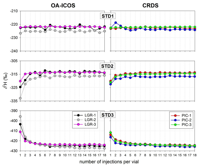
Fig. 1a. Measurement stabilisation by sequential injection number for three laboratory measurement standards (second triplet in an analysis run) for hydrogen. Left column: OA-ICOS instruments. Right column: CRDS instruments.
