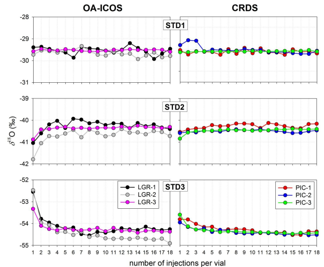
Fig. 1b. Measurement stabilisation by sequential injection number for three laboratory measurement standards (second triplet in an analysis run) for oxygen. Left column: OA-ICOS instruments. Right column: CRDS instruments.
