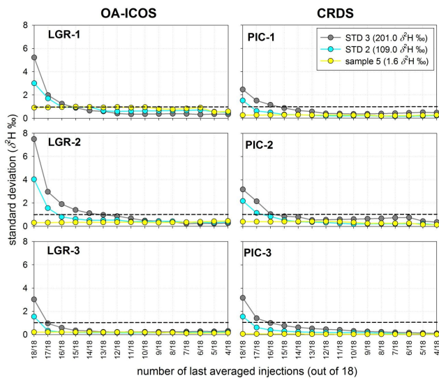
Fig. 4a. Standard deviation for \delta^2\text{H} for two laboratory measurement standards and one sample as a function of number of averaged injections. 18/18 indicates that all 18 injections of the same vial (either standard or sample) were averaged, whereas 17/18, 16/18, 15/18... indicates that only the last 17, 16, 15... injections were averaged (and the remaining discarded). The dotted horizontal line indicates currently acceptable reference precision for \delta^2\text{H} (1 ‰). The legend depicts the difference between the isotopic composition of the standard/sample displayed and the isotopic composition of the previous vial analysed in the tray.
