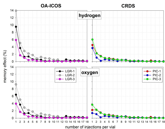
Fig. 2. MEs as a function of the number of sequential injections of the same vial for the transition between STD1 and STD3 (third triplet in an analysis run). Upper row: hydrogen. Lower row: oxygen. Left column: OA-ICOS instruments. Right column: CRDS instruments.
