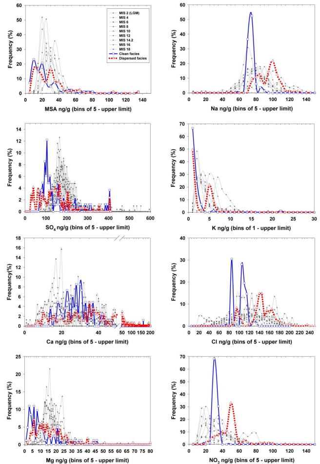
Figure 5. Frequency distribution of concentrations (in bins of 1 or 5 \text{ ngg}^{-1} or ppb) of selected chemical species in the clean (open blue squares – thick blue solid line) and dispersed (open red triangles – thick red dotted line) basal ice facies of the EPICA Dome C core, as compared to those for the preceding full glacial periods (incremented symbols and thin grey lines – courtesy of EPICA Chemistry Consortium). See text for definition of “full glacials”.
