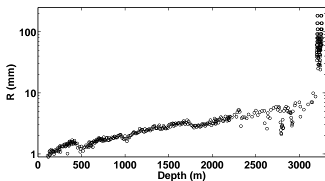
Figure 6. Mean equivalent crystals radii in the basal ice layers of the EPICA Dome C ice core, as compared to measurements in ice above 3200m depth from Durand et al. (2007). Basal ice measurements are preliminary results obtained using the linear intercept technique “on site”, while the data from above 3200m were obtained using automatic ice texture analyzers (AITAs – Wang and Azuma, 1999; Russell-Head and Wilson, 2001; Wilen et al., 2003).
