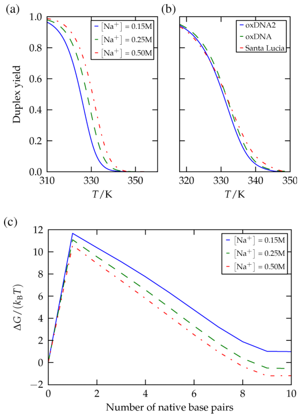
FIG. 7. The thermodynamics of formation of a 10-bp duplex with oxDNA2. (a) Duplex yield for oxDNA2 at different salt concentrations. (b) Comparison of duplex yield profiles at [\text{Na}^+] = 0.5\text{M} as predicted by oxDNA2, the original oxDNA model and the SantaLucia model. 49 (c) The free-energy profile for duplex formation at different salt concentrations, at the melting temperature of a 10-bp duplex at [\text{Na}^+] = 0.25\text{M} . The duplex was simulated for at least 3 \times 10^{10} virtual move Monte Carlo 76 (VMMC) steps at each salt concentration using umbrella sampling at a monomer concentration of 3.3 \times 10^{-4}\text{M} .
