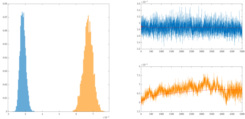
Figure 10: Posterior distribution ( left plot ) and MCMC output ( right plots ) of the quadratic norm of the tensor of coefficients, in regime 1 ( blue ) and regime 2 ( orange ).
