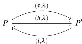
Figure 1: A simple two state model.
