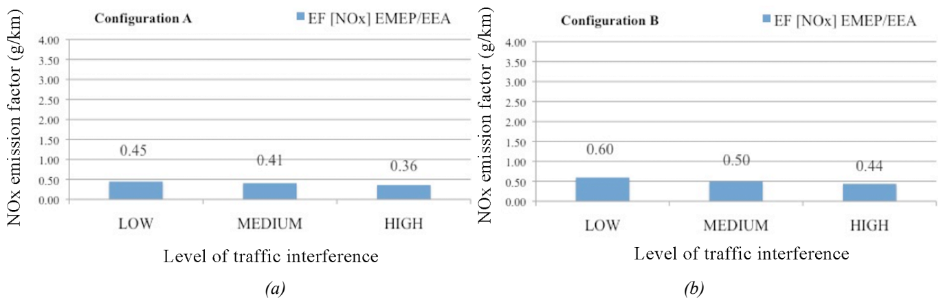
Fig. 5 – NO x emission factors (EF) calculated through the EMEP/EEA static method
