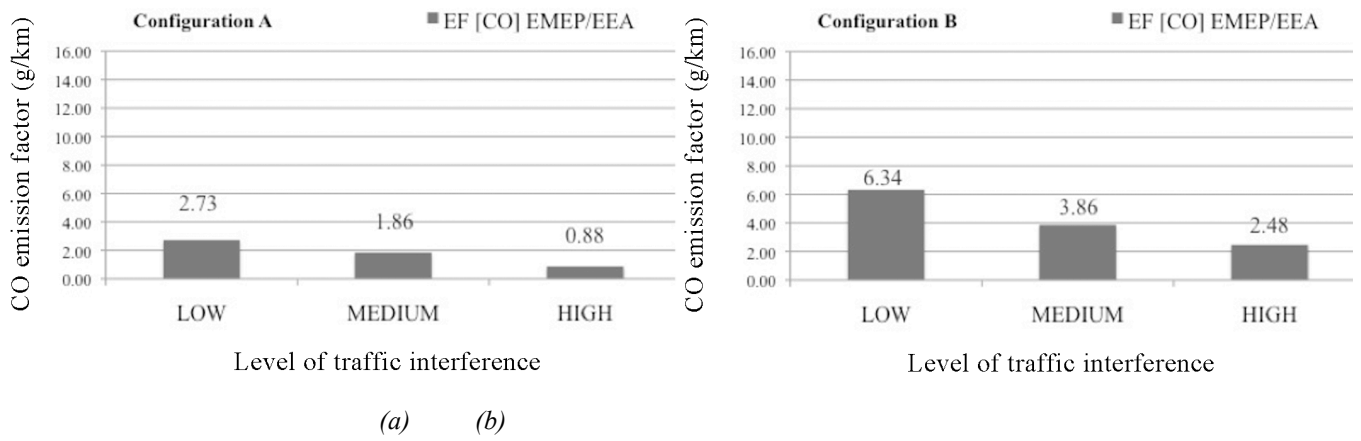
Fig. 4 – CO emission factors (EF) calculated through the EMEP/EEA static method
