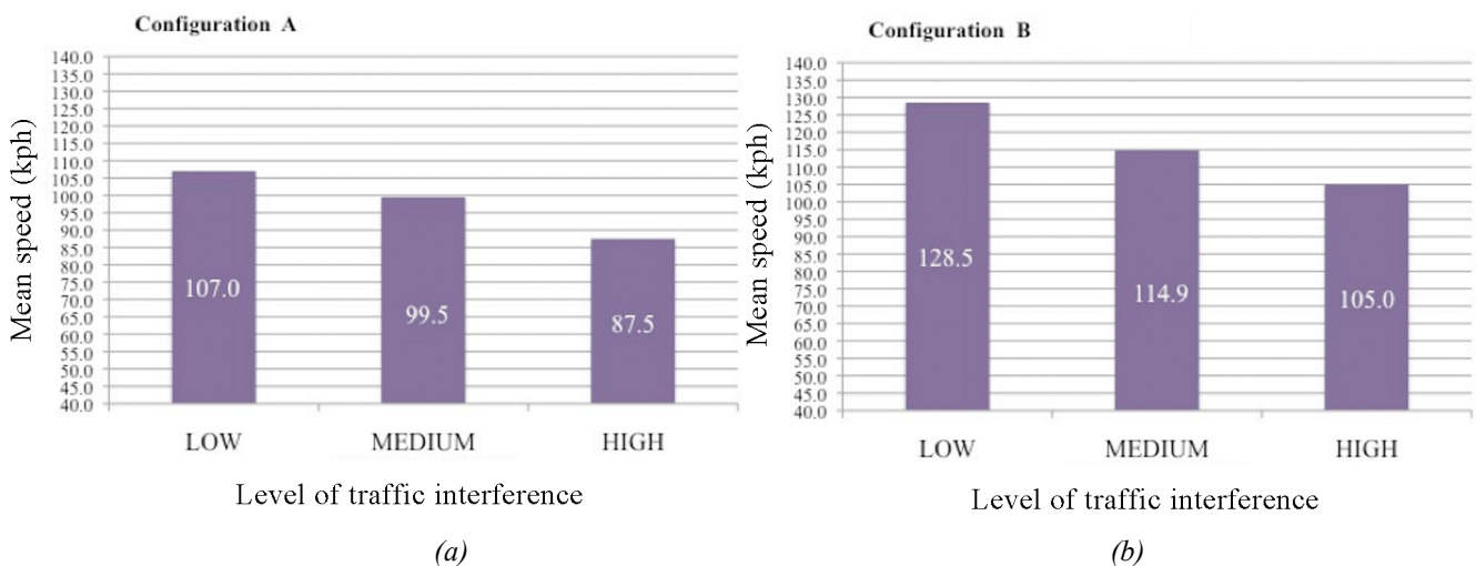
Fig. 6 – Mean speed levels in different traffic flow scenarios
