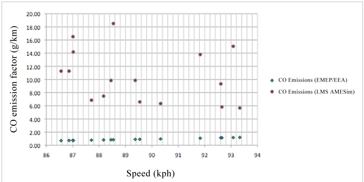
Fig. 2 – Difference between predicted and simulated emission factor values
