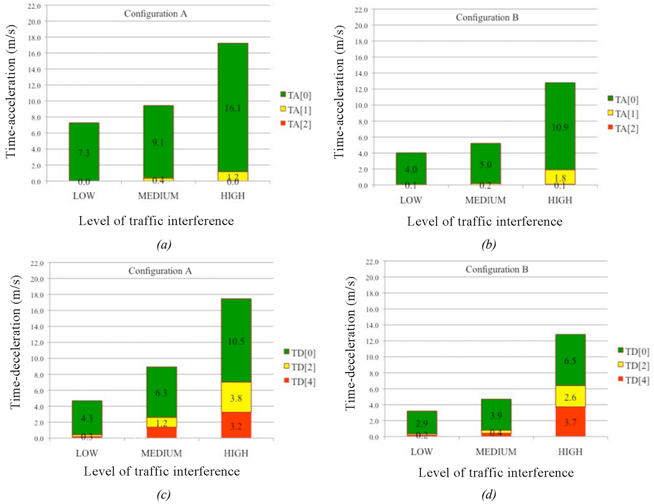
Fig. 3 – TA (a, b) and TD (c, d) values in configurations A and B
