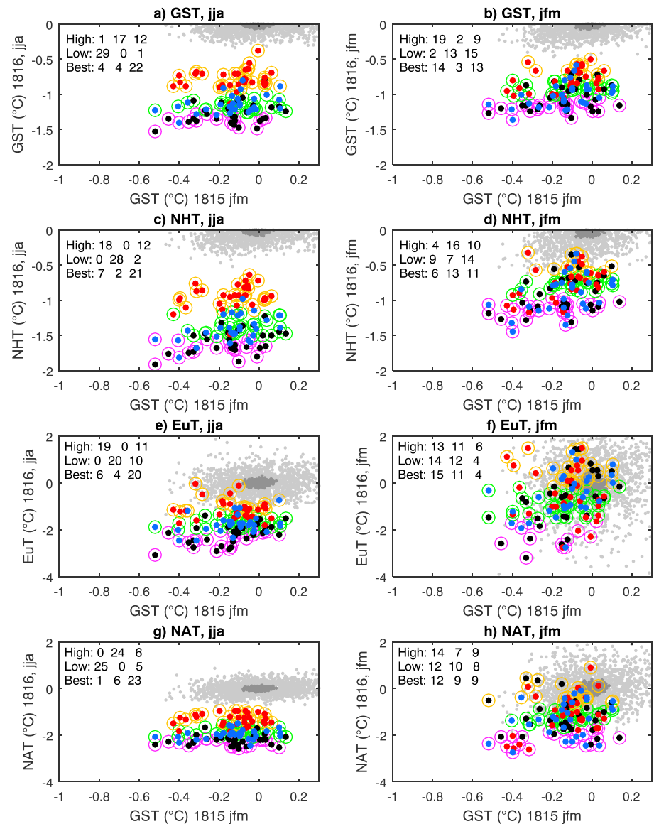
Figure 2. Scatterplot of surface temperature response (y axis) versus initial conditions (x axis) for (a, b) GST, (c, d) NHT, (e, f) EuT, and (g, h) NAT, for the summer 1816 (left column) and winter 1815/1816 (right column) responses. Small filled circles are the original ensembles (color code as in Figure 1); large empty circles are the clusters. The top three text lines in each panel report how the members of each of the original ensembles are redistributed across the clusters. The clouds of small gray dots show the range of variations that can be associated to internal variability through sampling along the control simulation (light: single simulation; dark: 30-member ensemble mean). GST = near-surface air temperatures spatially averaged over the whole globe; NHT = near-surface air temperatures spatially averaged over the Northern Hemisphere; EuT = near-surface air temperatures spatially averaged over Europe; NAT = near-surface air temperatures spatially averaged over North America.
