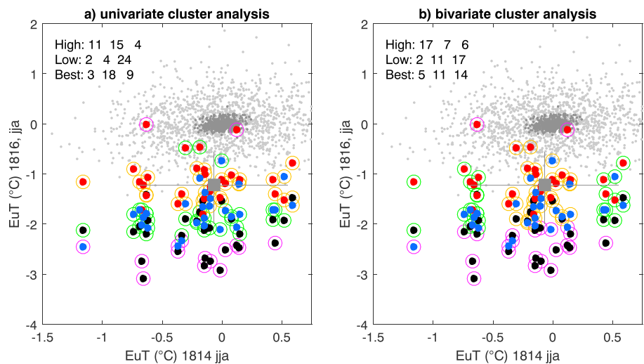
Figure 4. Scatterplot of climate response versus initial conditions for the 1816 EuT. Initial conditions are based on summer 1814 EuT anomalies. Clustering is performed on the difference between the simulated anomalies and the EuT reconstruction by Luterbacher et al. (2016), indicated by the gray square with associated uncertainty range (bars). (a) Cluster analysis on summer 1816 EuT anomalies alone (univariate); (b) cluster analysis on both summer 1816 EuT and summer 1814 EuT anomalies (bivariate). Representation as in Figure 2. Note that the data are the same in both panels, which differ only for the results of the clustering. EuT = near-surface air temperatures spatially averaged over Europe.
