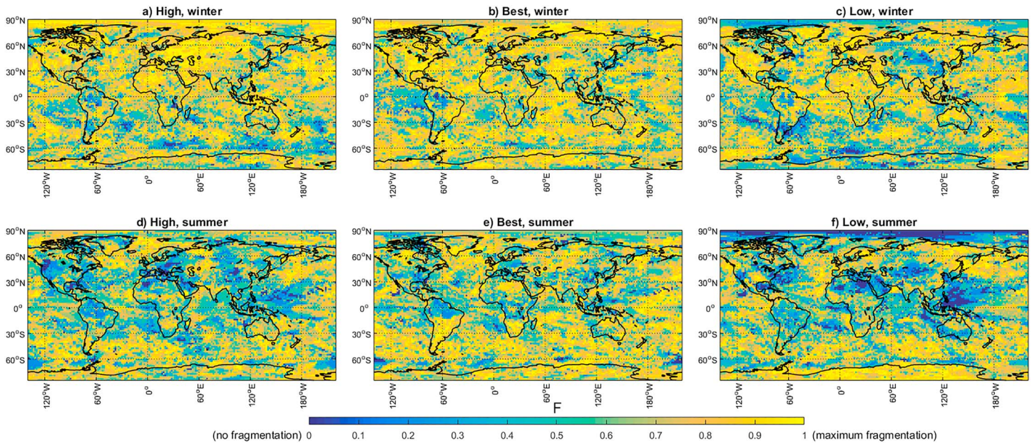
Figure 3. Fragmentation of grid point NH winter 1815/1816 (a–c) and summer 1816 (d–f) near-surface air temperature anomalies from the preeruption (1810–1814) climatology in the (a, d) High, (b, e) Best, and (c, f) Low ensembles.
