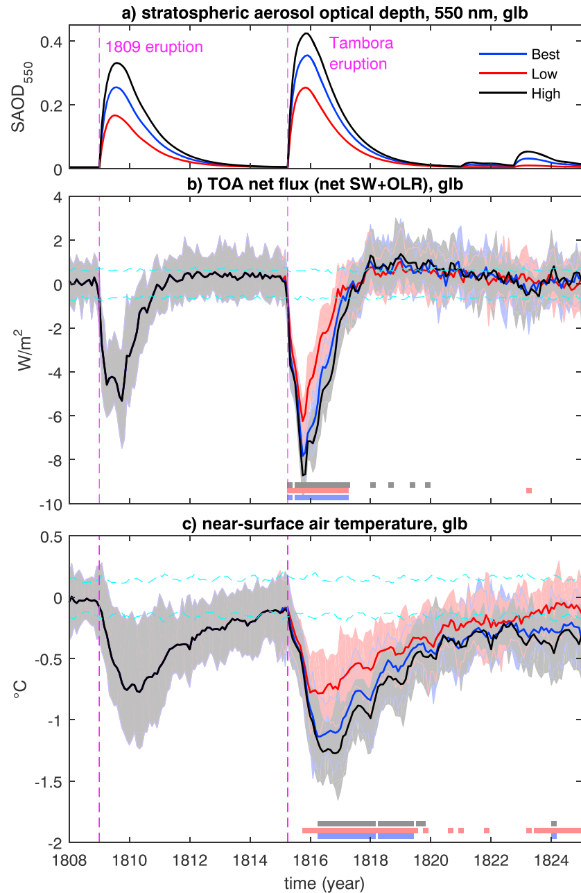
Figure 1. (a) Global-average monthly stratospheric aerosol optical depth at wavelength 550 nm produced by Easy Volcanic Aerosol v1.0; (b, c) ensemble mean (lines) and 5th–95th percentile intervals (shading) of global-mean top-of-atmosphere net radiative flux (positive means downward) and near-surface air temperature anomalies. Monthly anomalies are deviations from the respective climatology over the period 1800–1808. The three ensembles overlap by construction before 1815. Turquoise dashed lines are the 5th–95th percentile intervals for signal occurrence in the control run. Bottom rectangles indicate periods when an ensemble (color code as for the time series plots) is significantly different ( p = 0.05 ) from both the other two ensembles according to the Mann-Whitney U test. SAOD = stratospheric aerosol optical depth; TOA = top-of-atmosphere; SW= shortwave radiation; OLR= outgoing longwave radiation.
