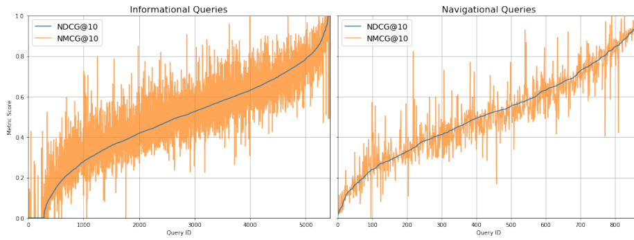
Fig. 2 Comparison of nDCG@10 vs. nMCG@10 score distributions for informational and navigational queries.
