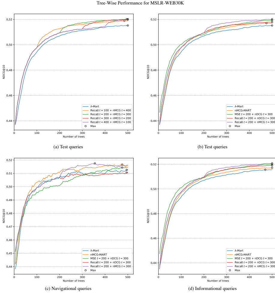
Fig. 3 Comparison of continuation methods approaches trained with nMCG and with different switching points (a) and comparison of different models on test queries (b), just on navigational queries (c) and just on informational queries (d). All the figures refers to MSLR-WEB30K Fold 1 and all the models are evaluated with respect to nDCG@10.
