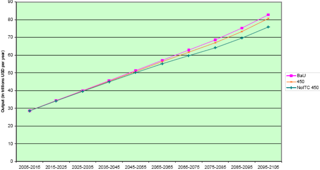
Figure 5: The GDP Cost of Stabilising GHG Concentrations at 450 ppm with and without Induced Technical Change
